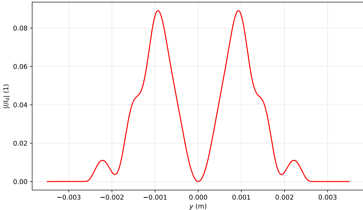
Intensity profile I(x=0, y, z=3.981)/I_0 , P_{in}=4.0P_{cr} , artificial time
